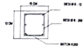
DETAIL BALOK 15X12
